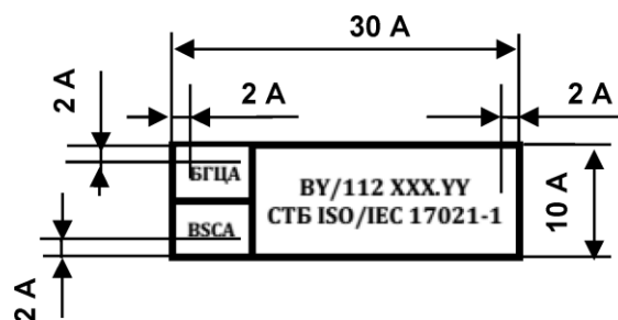
Figure 3.2 - The ratio of the minimum margins on overall linear dimensions accreditation symbol
