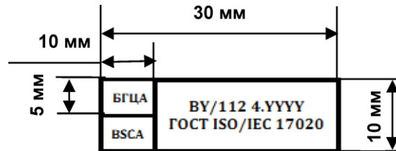
Figure 3.1 - Basic dimensions of accreditation symbol
